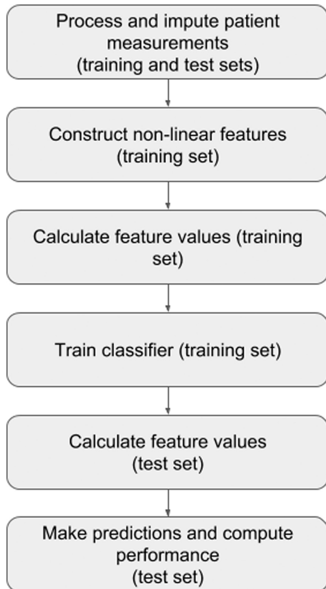
Fig. 2. AutoTriage algorithm flowchart.
